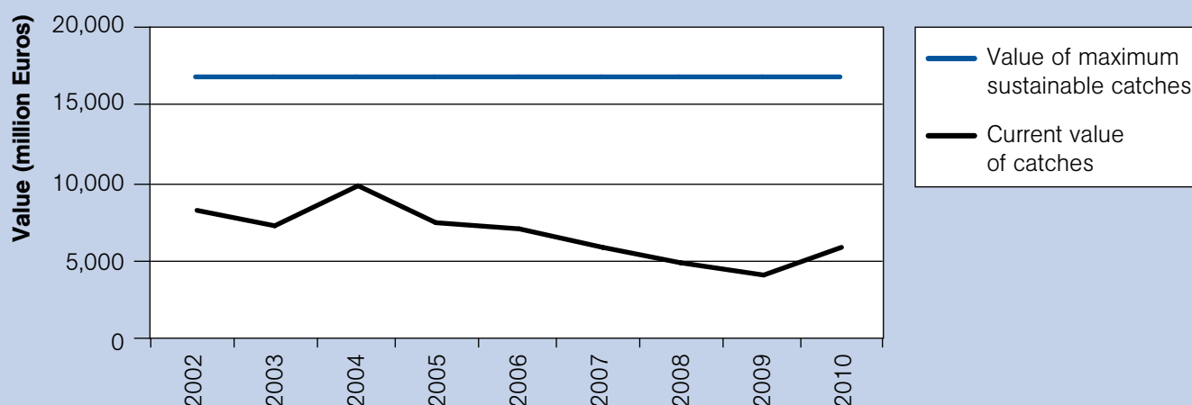
Figure 3: The current value of catches from 54 fish stocks are shown relative to their sustainable maximum. MSY values are in 2011 prices, while current values are nominal. Source: MSY estimates from Froese & Proelß 26 and current value of catches are own calculations based on ICES stock assessments and the AER. 27 See technical appendix for methods.
