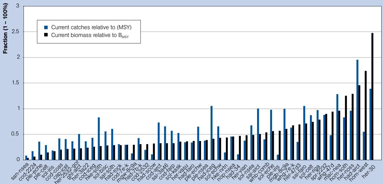
Figure A1: Current biomass ( B_{MSY} ) and catches relative to their respective maxima (BMSY and MSY) for all 54 stocks. Data sources. 67,68
