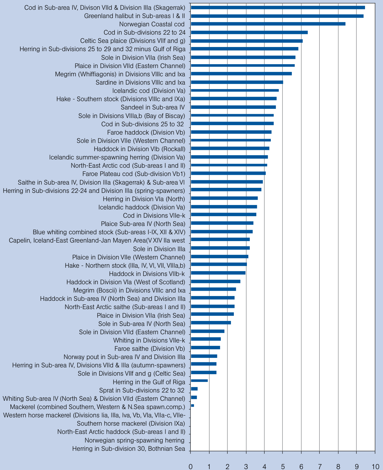
Figure 4: Time taken to restore fish stocks. If fishing stopped on 1 January 2013 (= time 0) then it would take around 1 year for herring in the Gulf of Riga to recover. The rebuilding time of the 54 stocks depends on their current size (spawning stock biomass (SSB)) and their potential size (BMSY), while assuming that their growth is logistic in nature. See the technical appendix for details. Of the 54 fish stocks in this study, 49 are below their BMSY level, and five are above: two herring stocks (her-30 and her-noss), one haddock stock (had-arct), and two mackerel stocks (hom-soth and hom-west).
